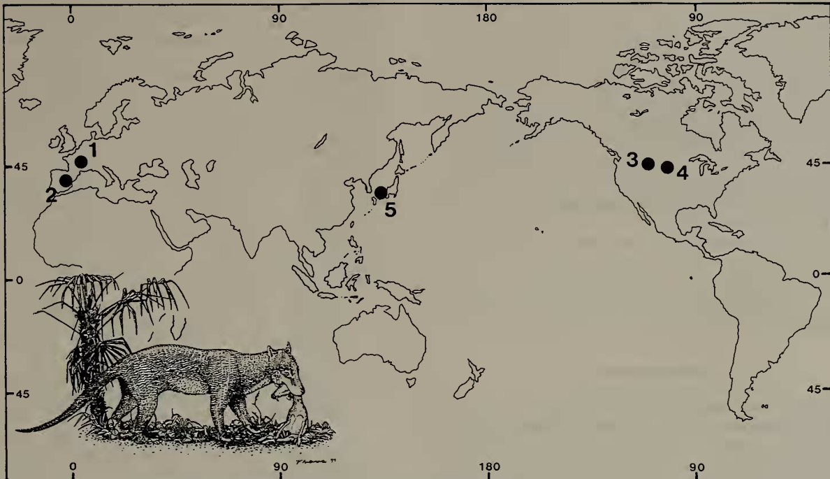
Figure 2. Distribution of Ysengrinia . 1, Y. tolosana , Late Oligocene; Y. gerandiana , early Early Miocene; Y. depereti , late Early Miocene, France. 2, Y. valentiana , late Early Miocene, Spain. 3, Y. sp. , Early Miocene, Wyoming, U.S.A. 4, Y. sp. , Early Miocene, Nebraska, U.S.A. 5, Y. sp. , early Middle Miocene, Japan. Illustration is a generalized life restoration of an amphicyonid.
